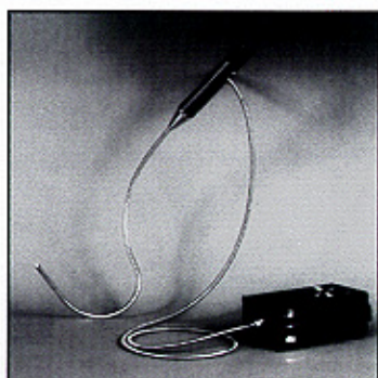
General Purpose Flexible Borescope (P/N FFSL1) shown with 100 watt Light Source (P/N LSP1)
